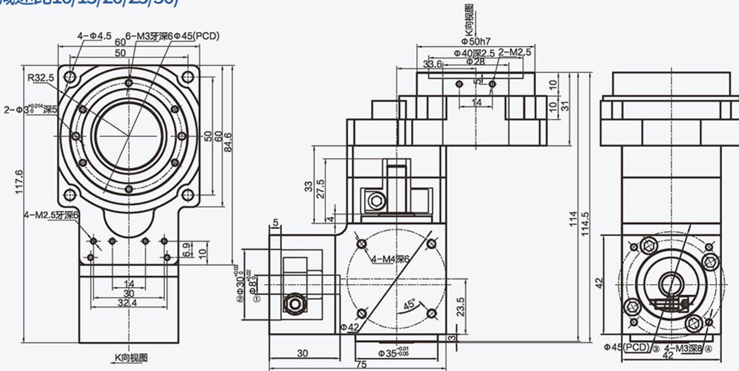
AK60-Z (減速比10/15/20/25/50)
