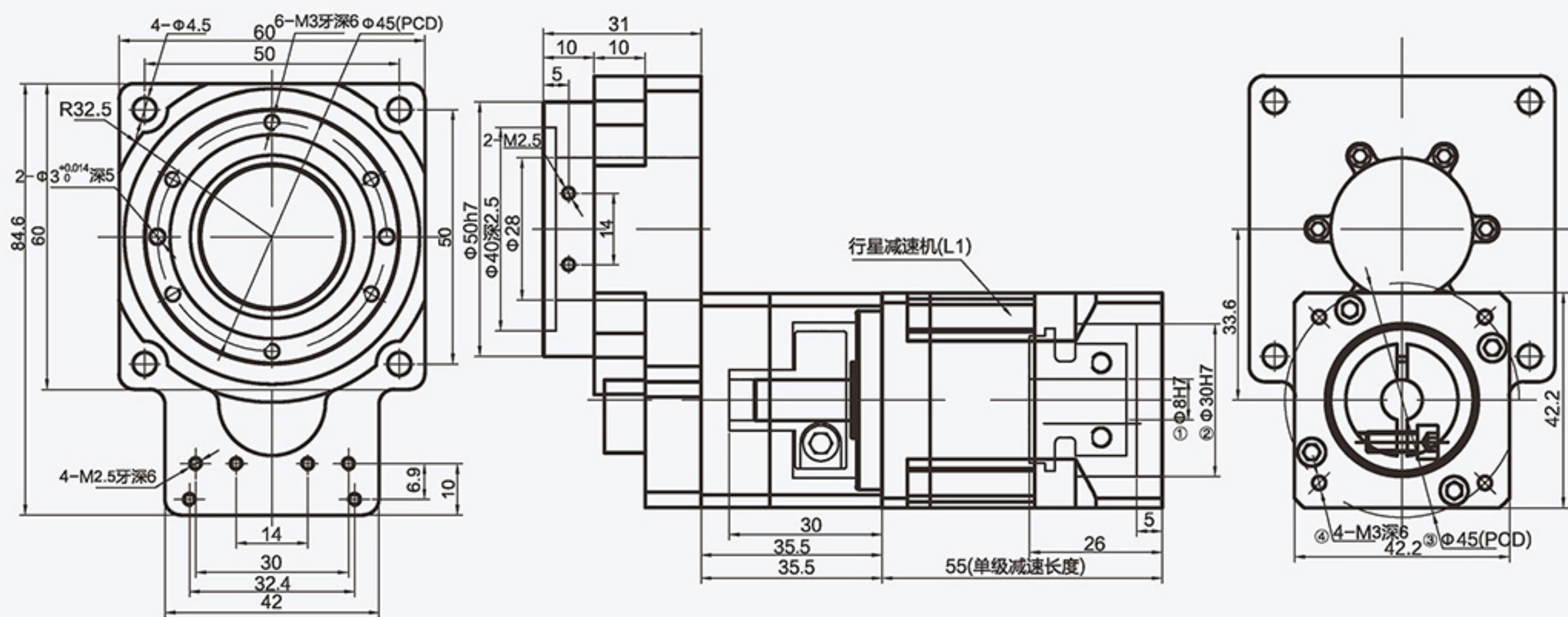
AK60-F (減速比15/20/25/35/40/50)
